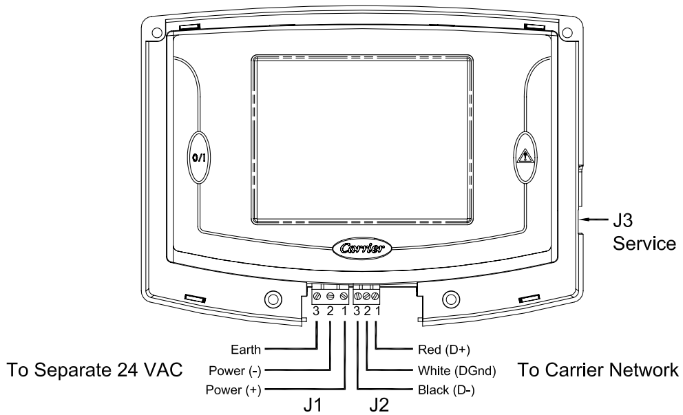
Figure 4 — Touch Pilot Surface Mounting
